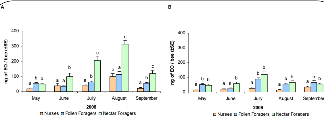
Figure 4: EO amount during seasons 2008 (A) and 2009 (B) in nurses, pollen and nectar foragers. a, b, c denote significant differences P<0.05 between the three group of bee each month.
