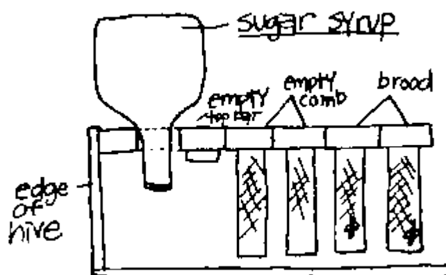
Feeder for KTBH (long side view)
