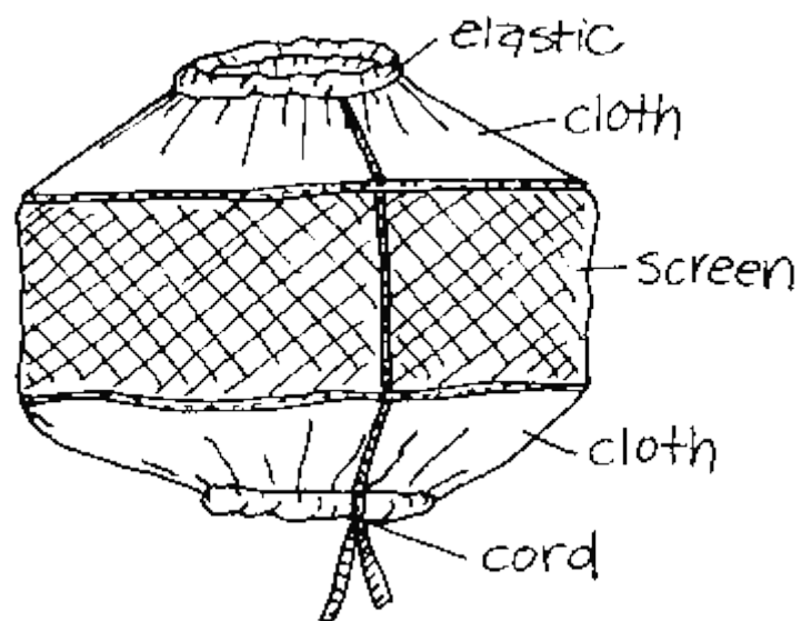
Solar wax melter
