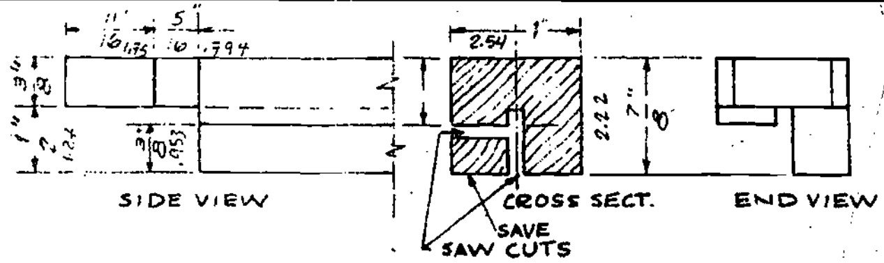
FULL SIZE DETAIL FRAME TOP
