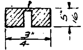
CROSS SECTION FULL SIZE
